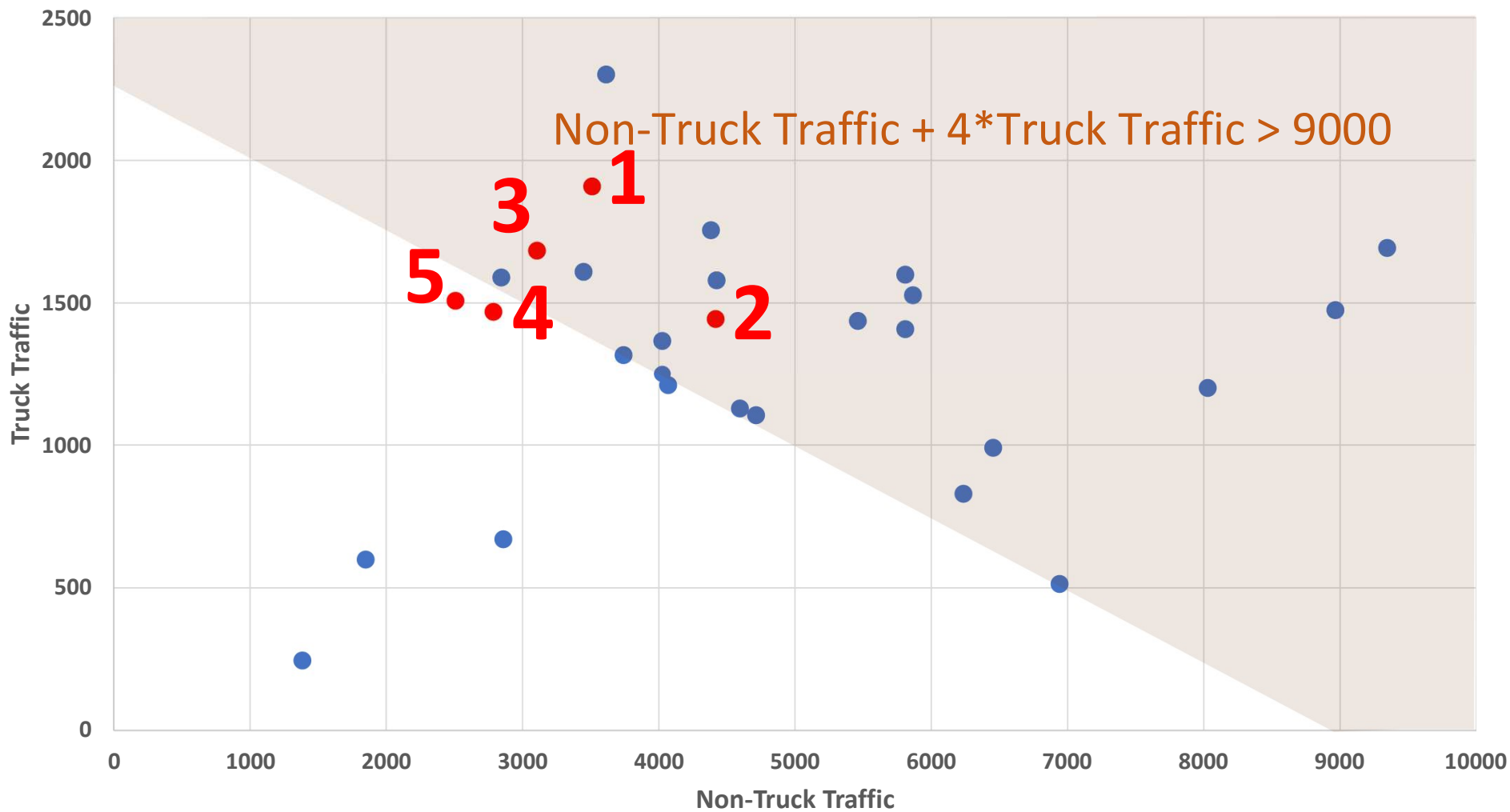
Average Total vs Truck Traffic on Divided Non-Urban Highways
